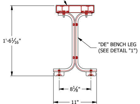
RUBBER FOOT PAD OPTION SEE DETAIL "2"
