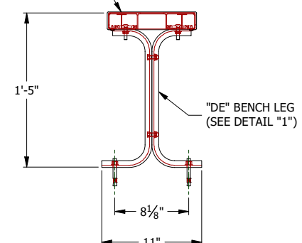
CONCRETE ANCHORED OPTION SEE DETAIL "3"
